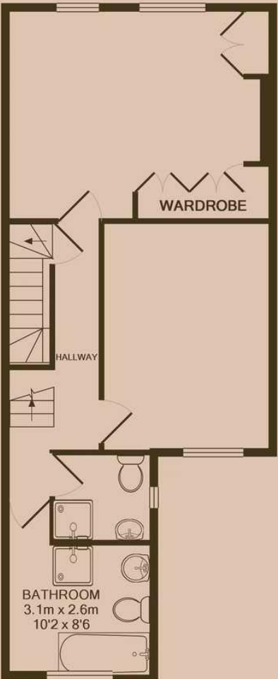
1ST FLOOR
